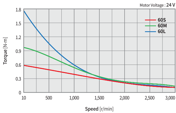
Ezi-SERVO-CT-ALL-60 series
