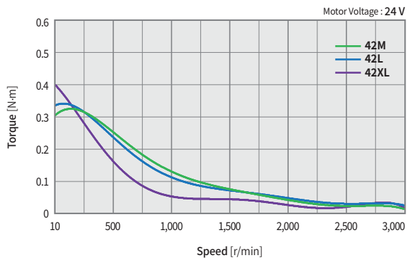
Ezi-SERVO-CT-ALL-42 series
