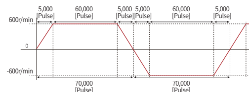
Condition to measure the motor temperature
