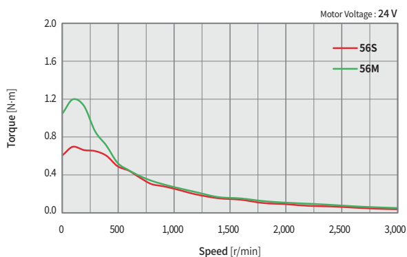
Ezi-SERVO-CT-4X-HSP56 series
