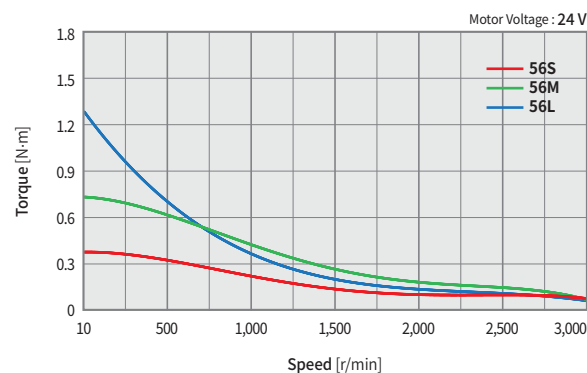
Ezi-SERVO-CT-4X-56 series
