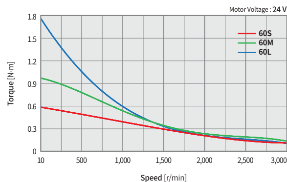
Ezi-SERVO-CT-4X-60 series
