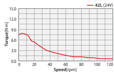
42L-PN25 Series
