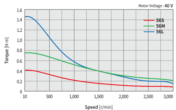
Ezi-STEP-CT-56 Series
