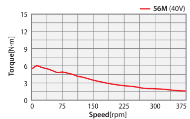
56M-PN25 Series
