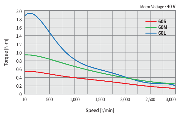
Ezi-STEP-CT-60 Series
