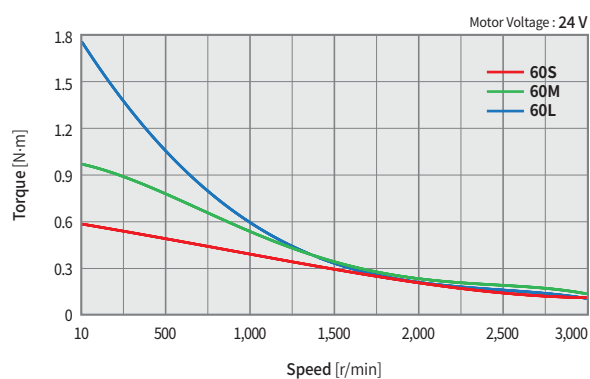
Ezi-STEP-CT-4X-60 series
