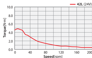
42L-PN50 Series
