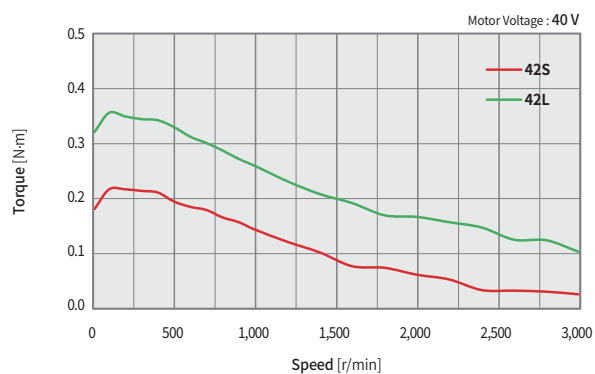
Ezi-SERVO-CT-HSP42 series
