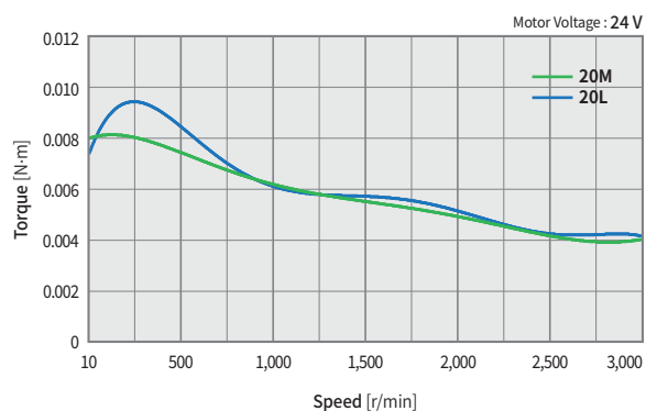
Ezi-SERVO-CT-35 Series
