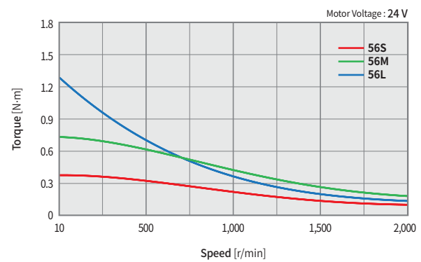
Ezi-SERVO-CT-ALL-56 series
