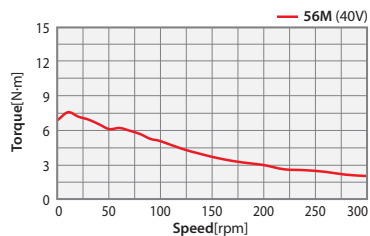
56M-PN40 Series
