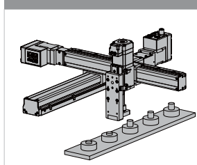
Component Assembly System
