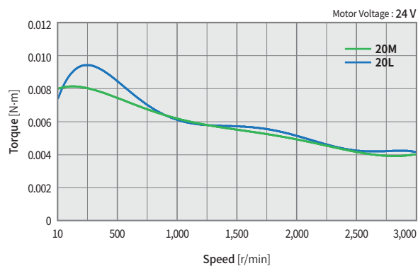
Ezi-STEP-CT-4X-42 series
