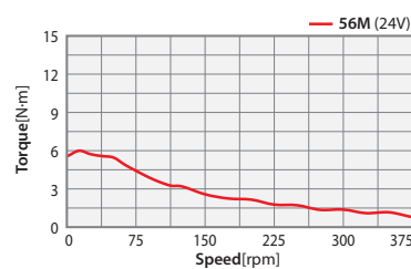
56M-PN25 Series
