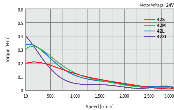
Ezi-SERVO-CT-4X-60 series
