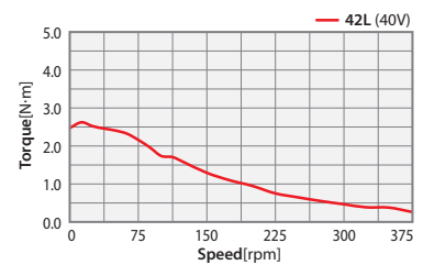
42L-PN25 Series
