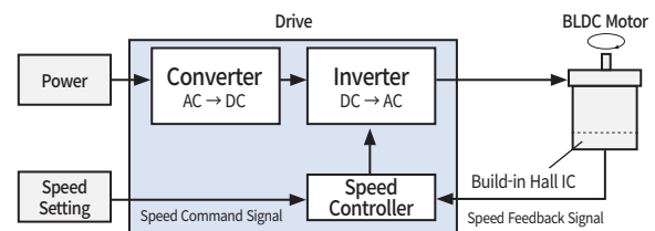
< Control Block Diagram >
