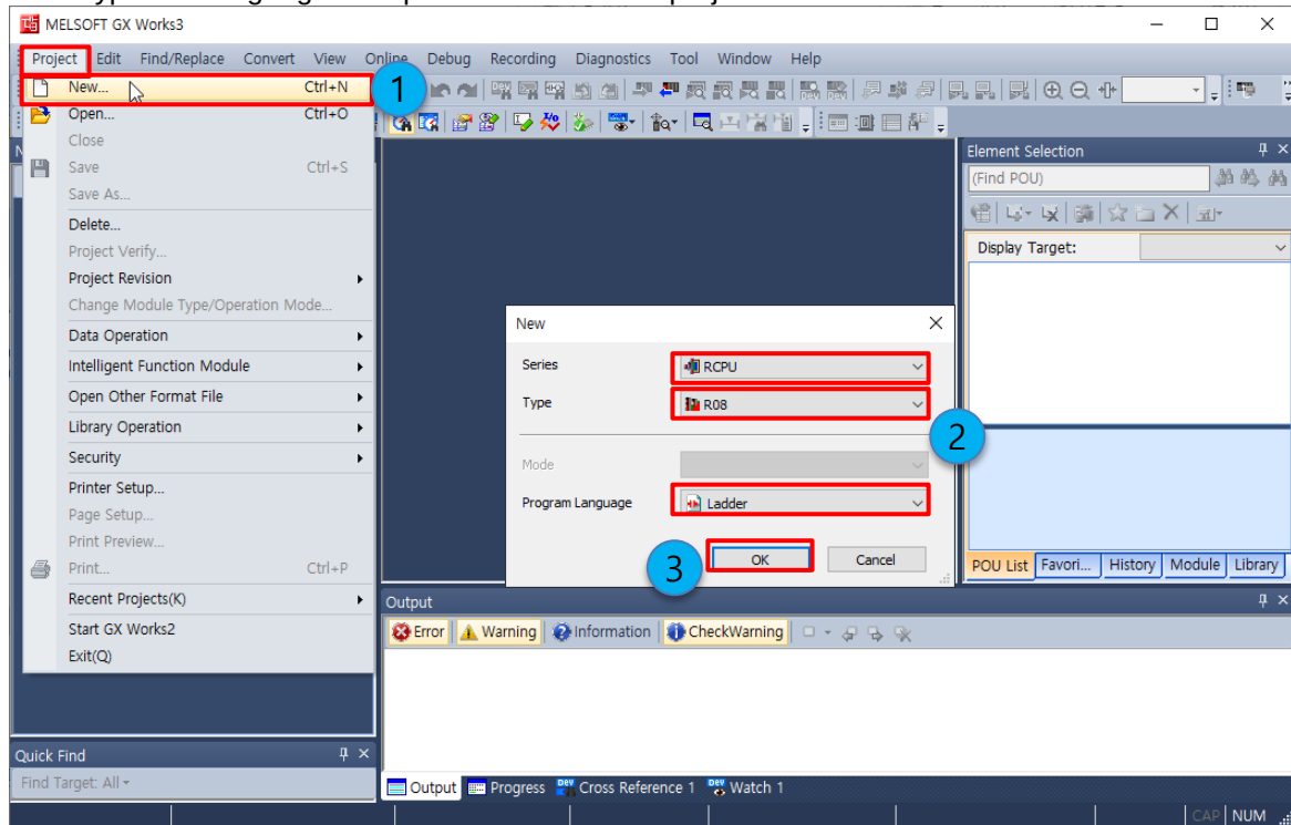
Figure 9-5. Create project
