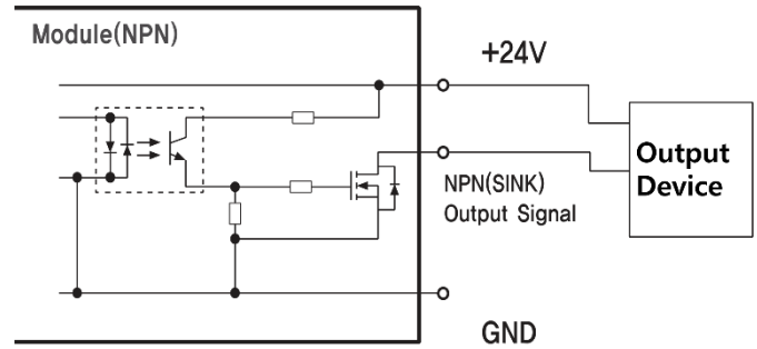
Figure 8-5. Example of NPN output 2-wire wiring
