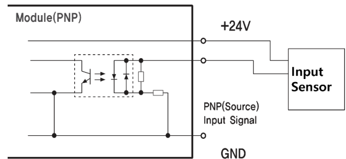
Figure 8-11. Example of PNP input 2-wire wiring
