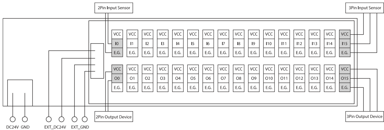
Figure 5-4. Ezi-IO-CT-I16O16N-E
