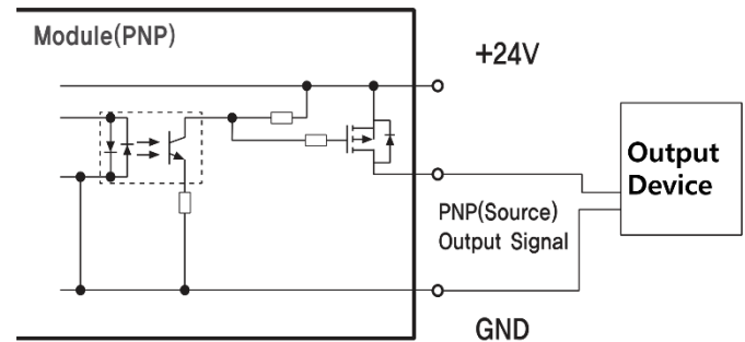
Figure 8-7. Example of PNP output 2-wire wiring
