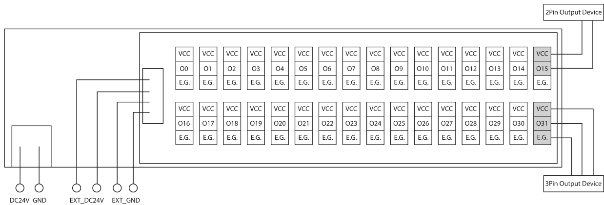
Figure 5-3. Ezi-IO-CT-O32N-E
