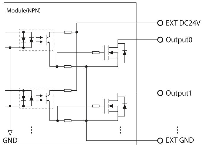
Figure 5-6. NPN output internal circuit diagram
