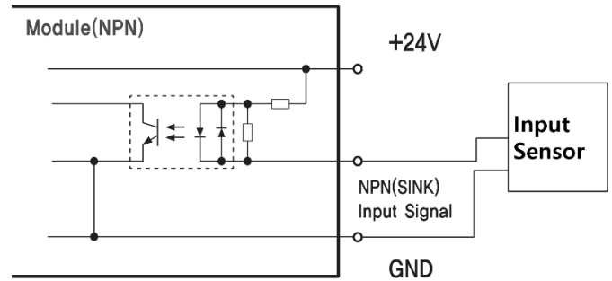
Figure 8-9. Example of NPN input 2-wire wiring
