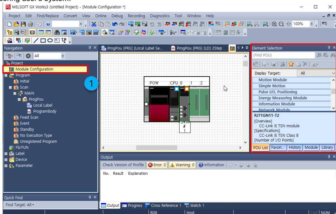
Figure 9-6. Set module.
