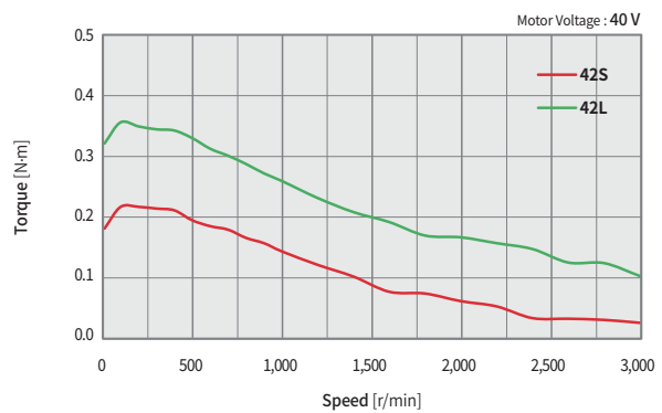
Ezi-SERVO-CT-HSP42 series
